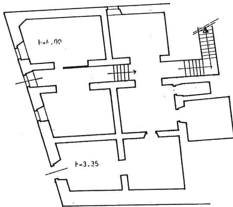
PIANO SEMINTERRATO
